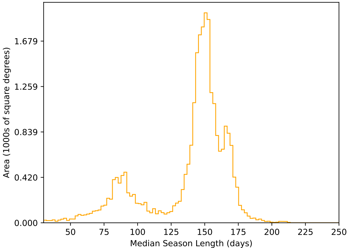
noroll_mjdp60_v3.4_10yrs All sky r band: Median Season Length
