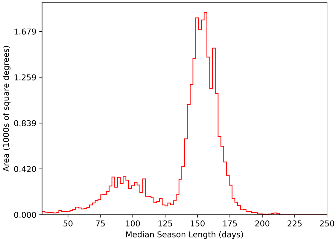
noroll_mjdp60_v3.4_10yrs All sky i band: Median Season Length
