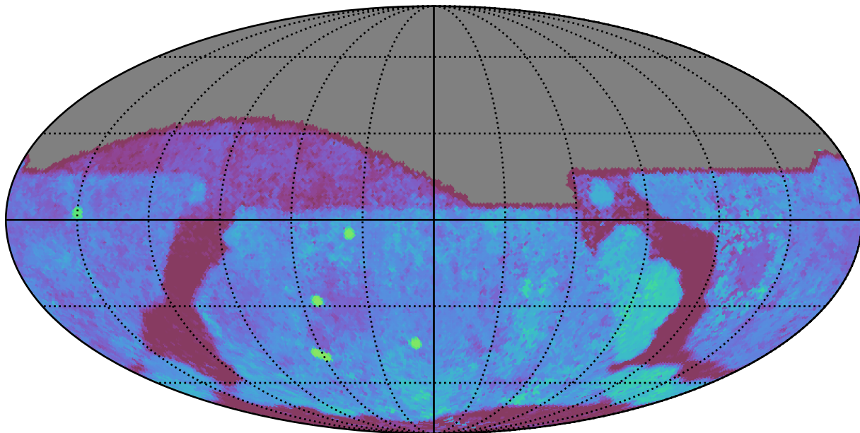
noroll_mjdp60_v3.4_10yrs All sky g band: Median Season Length
