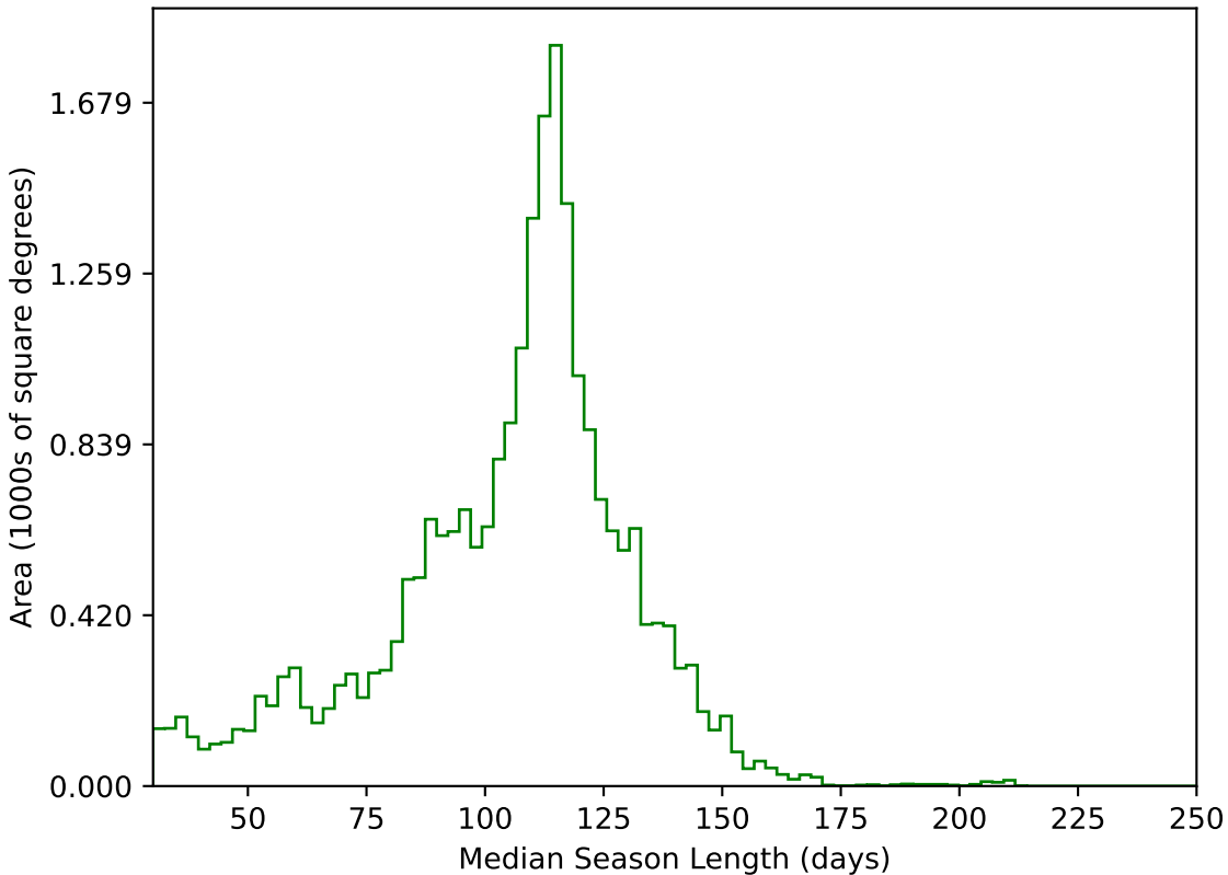
noroll_mjdp60_v3.4_10yrs All sky g band: Median Season Length
