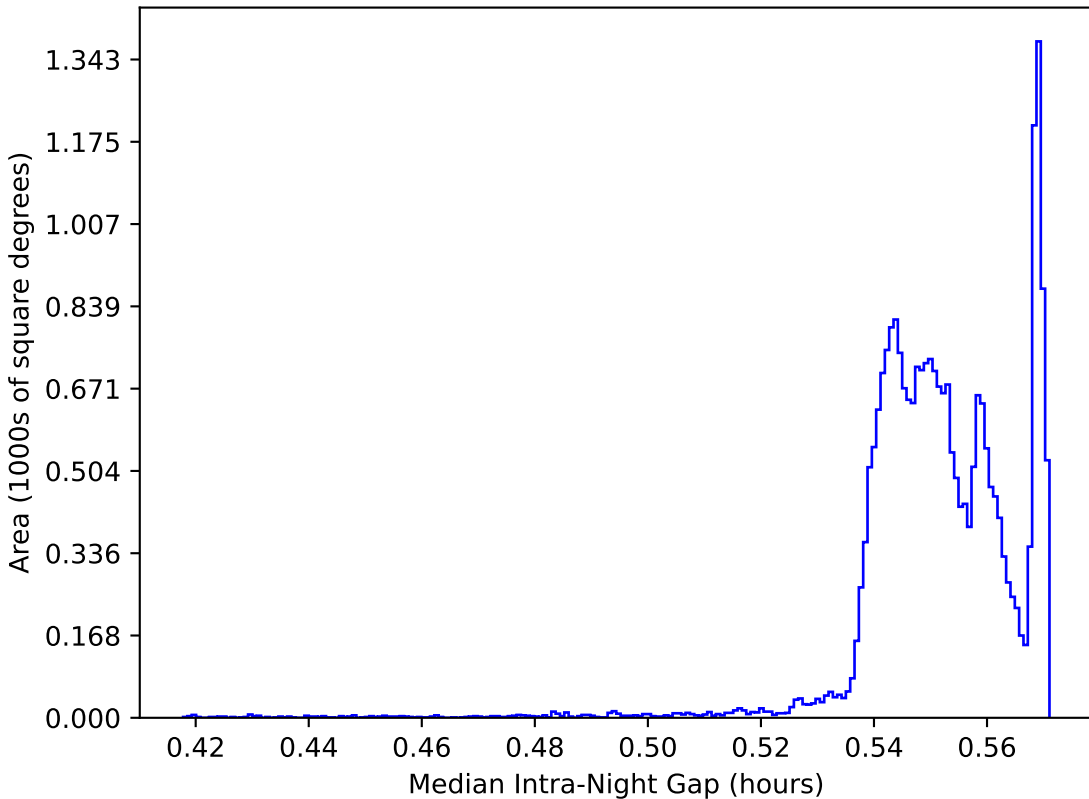
noroll_mjdp60_v3.4_10yrs All sky: Median Intra-Night Gap
