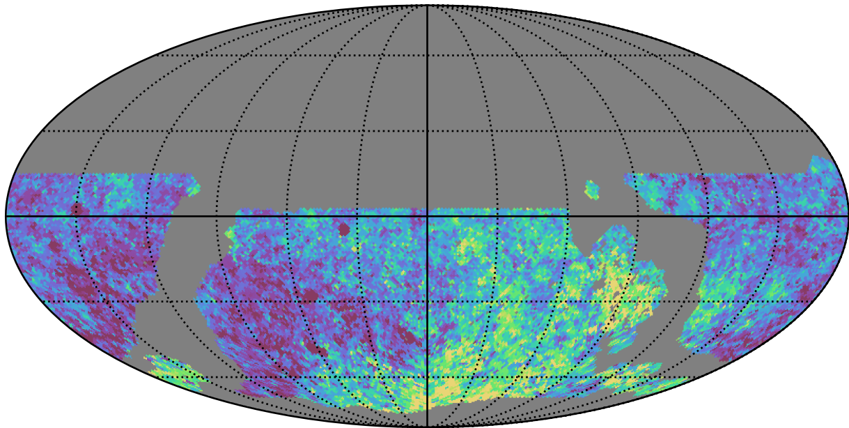
noroll_mjdp60_v3.4_10yrs WFD z band: Median Inter-Night Gap
