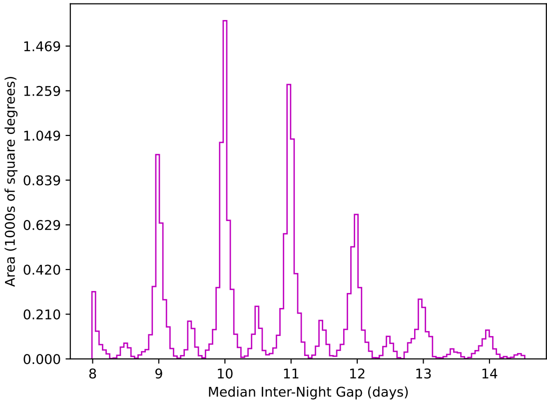
noroll_mjdp60_v3.4_10yrs WFD z band: Median Inter-Night Gap
