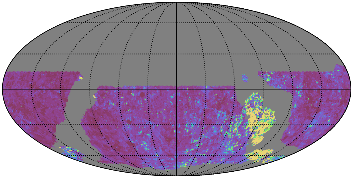
noroll_mjdp60_v3.4_10yrs WFD u band: Median Inter-Night Gap
