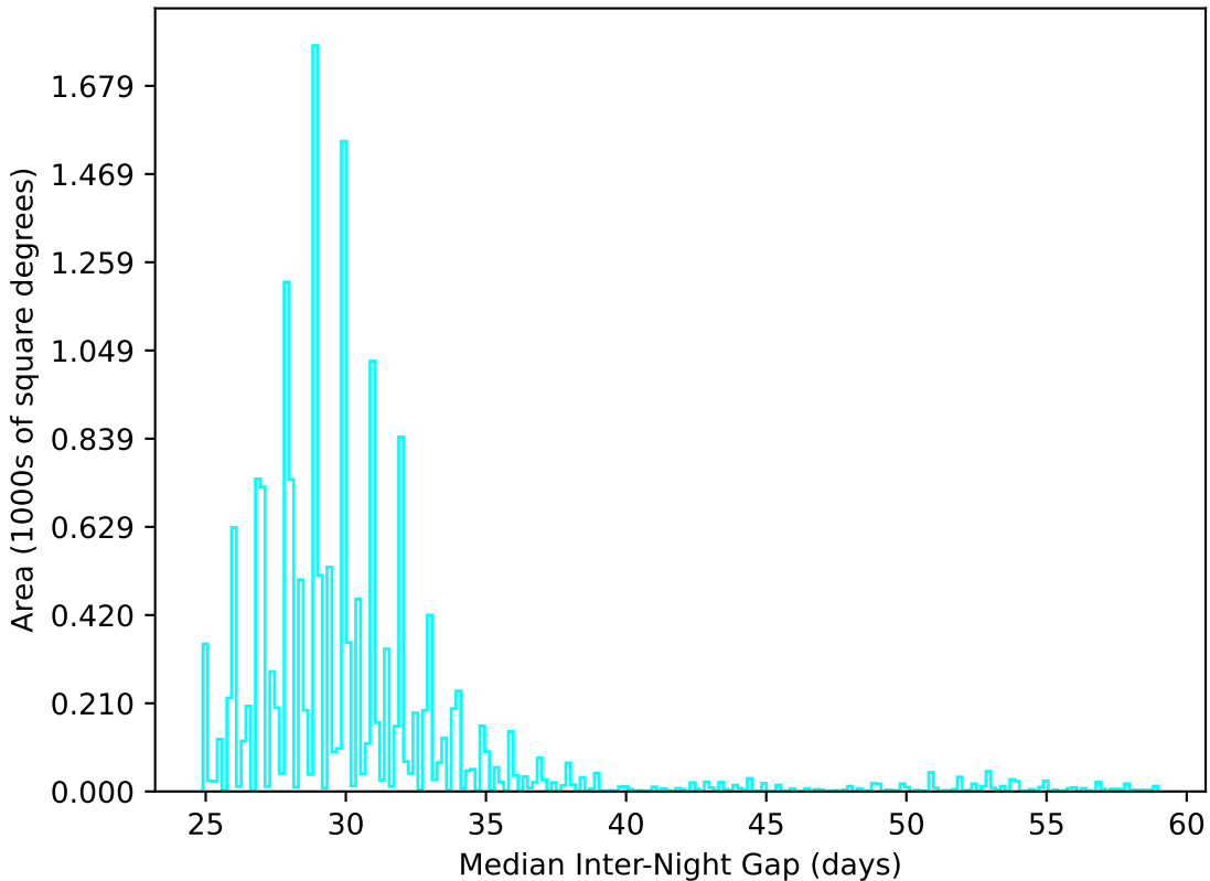
noroll_mjdp60_v3.4_10yrs WFD u band: Median Inter-Night Gap
