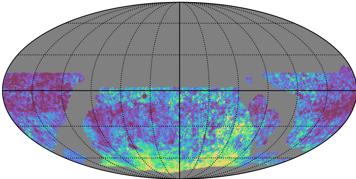
noroll_mjdp60_v3.4_10yrs WFD r band: Median Inter-Night Gap
