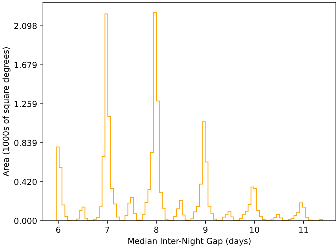
noroll_mjdp60_v3.4_10yrs WFD r band: Median Inter-Night Gap
