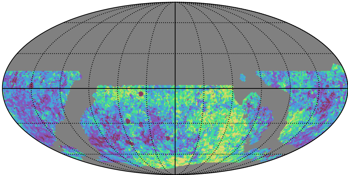
noroll_mjdp60_v3.4_10yrs WFD i band: Median Inter-Night Gap
