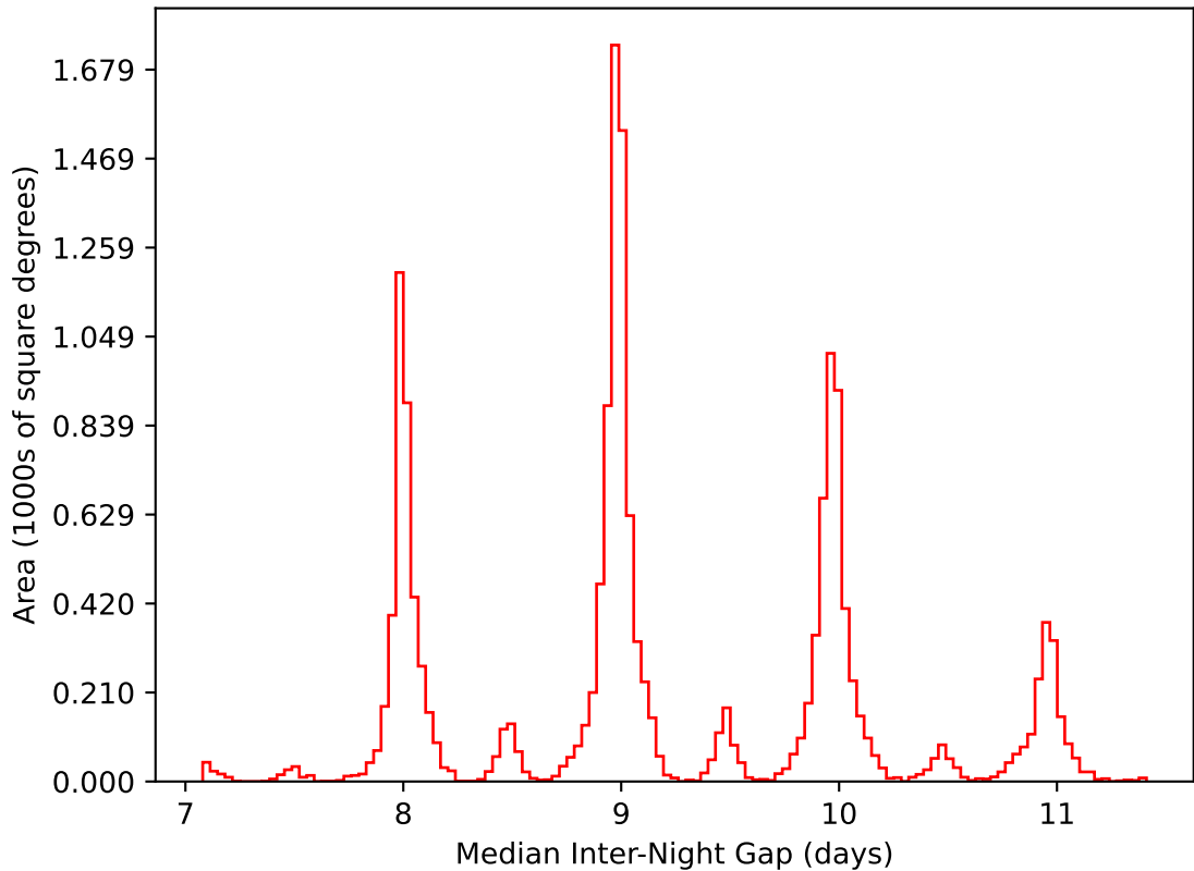
noroll_mjdp60_v3.4_10yrs WFD i band: Median Inter-Night Gap
