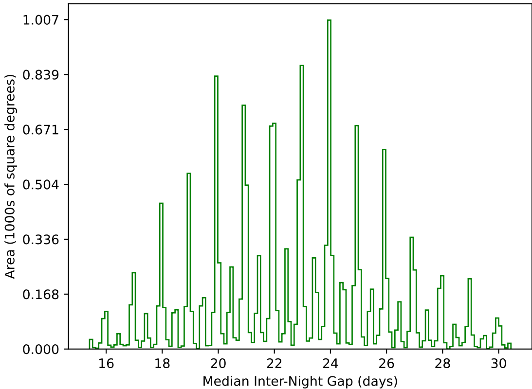
noroll_mjdp60_v3.4_10yrs WFD g band: Median Inter-Night Gap
