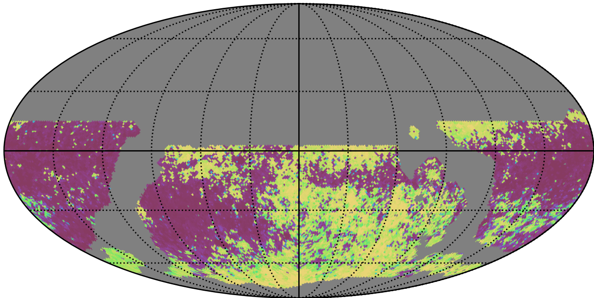
noroll_mjdp60_v3.4_10yrs WFD all bands: Median Inter-Night Gap
