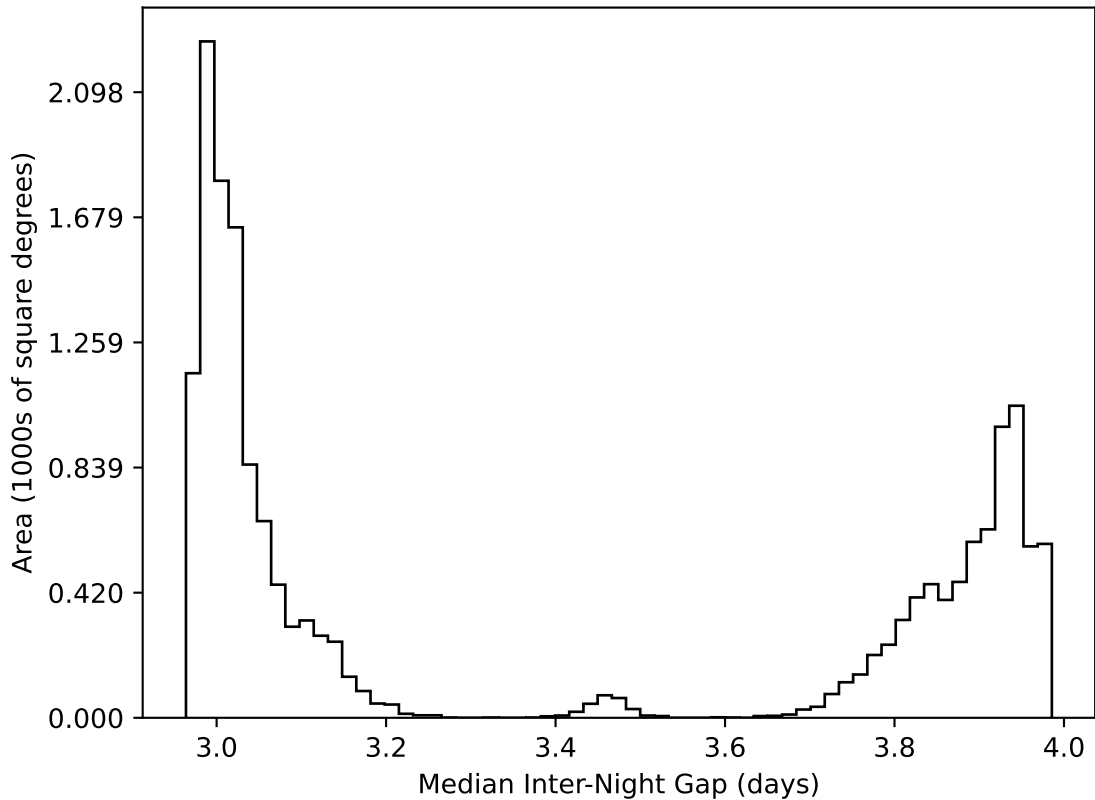
noroll_mjdp60_v3.4_10yrs WFD all bands: Median Inter-Night Gap
