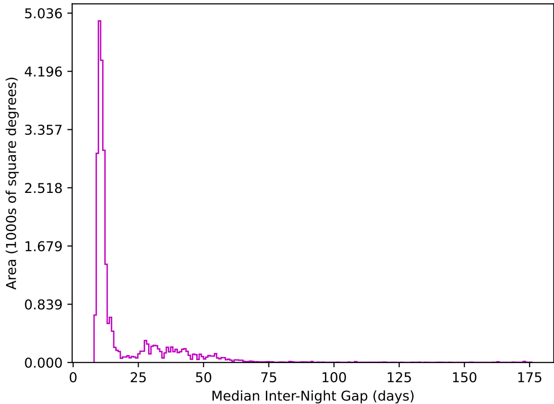
noroll_mjdp60_v3.4_10yrs All sky z band: Median Inter-Night Gap
