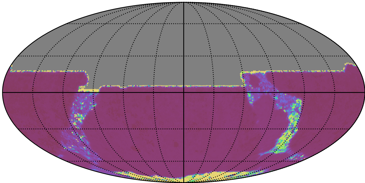
noroll_mjdp60_v3.4_10yrs All sky y band: Median Inter-Night Gap
