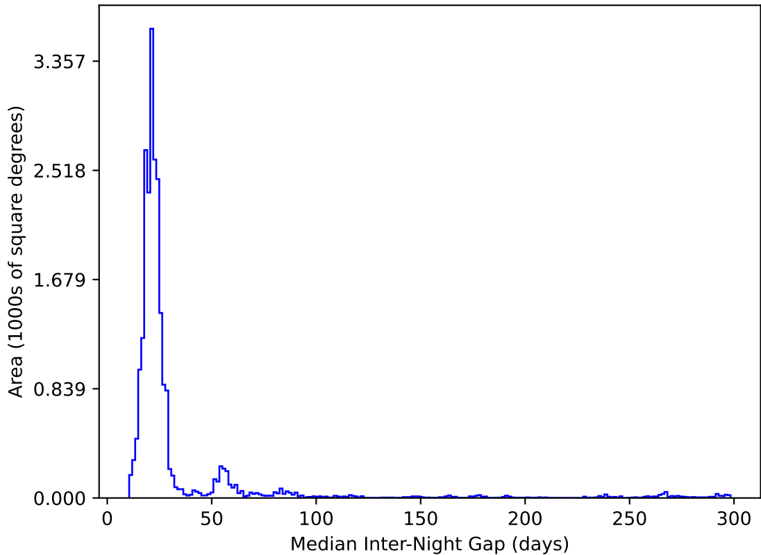
noroll_mjdp60_v3.4_10yrs All sky y band: Median Inter-Night Gap
