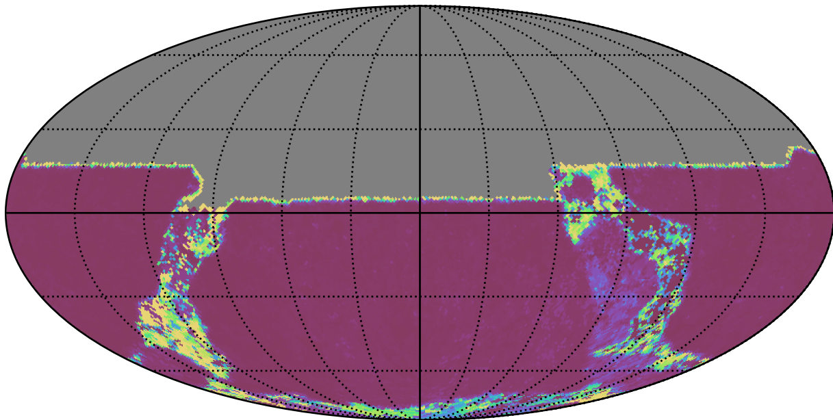
noroll_mjdp60_v3.4_10yrs All sky u band: Median Inter-Night Gap
