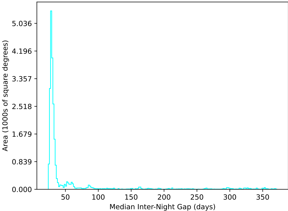
noroll_mjdp60_v3.4_10yrs All sky u band: Median Inter-Night Gap
