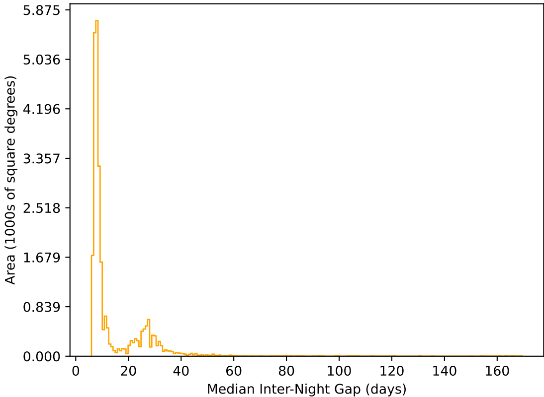
noroll_mjdp60_v3.4_10yrs All sky r band: Median Inter-Night Gap
