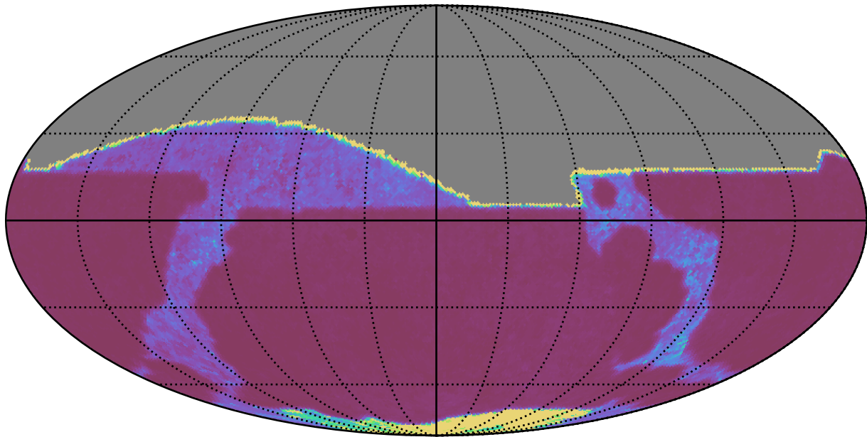
noroll_mjdp60_v3.4_10yrs All sky i band: Median Inter-Night Gap
