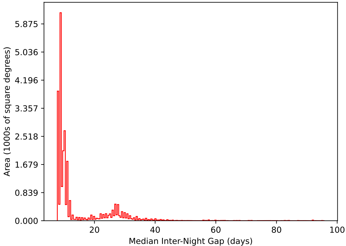
noroll_mjdp60_v3.4_10yrs All sky i band: Median Inter-Night Gap
