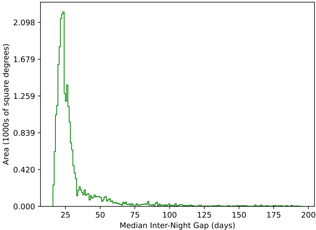
noroll_mjdp60_v3.4_10yrs All sky g band: Median Inter-Night Gap
