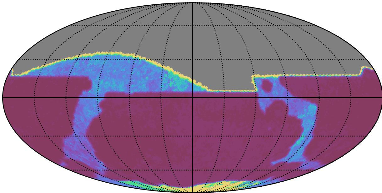
noroll_mjdp60_v3.4_10yrs All sky all bands: Median Inter-Night Gap
