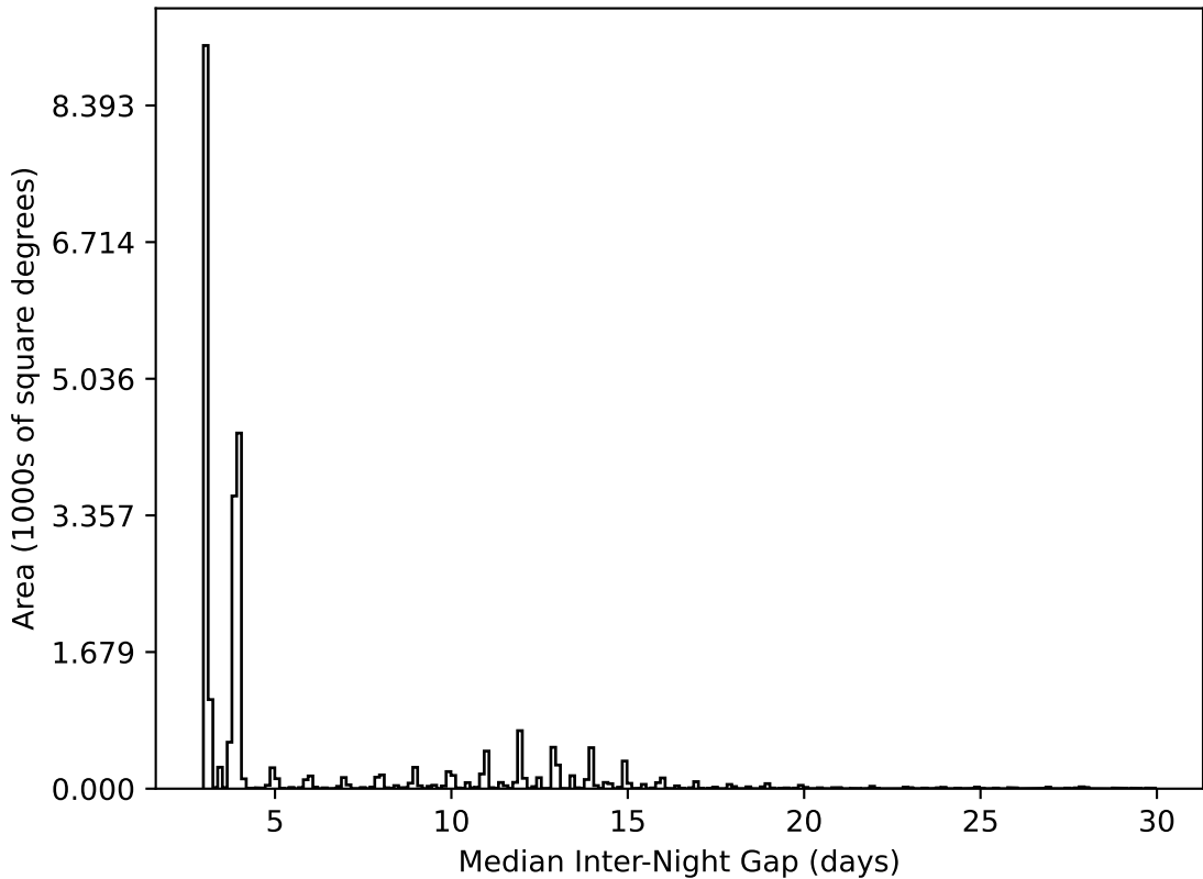
noroll_mjdp60_v3.4_10yrs All sky all bands: Median Inter-Night Gap
