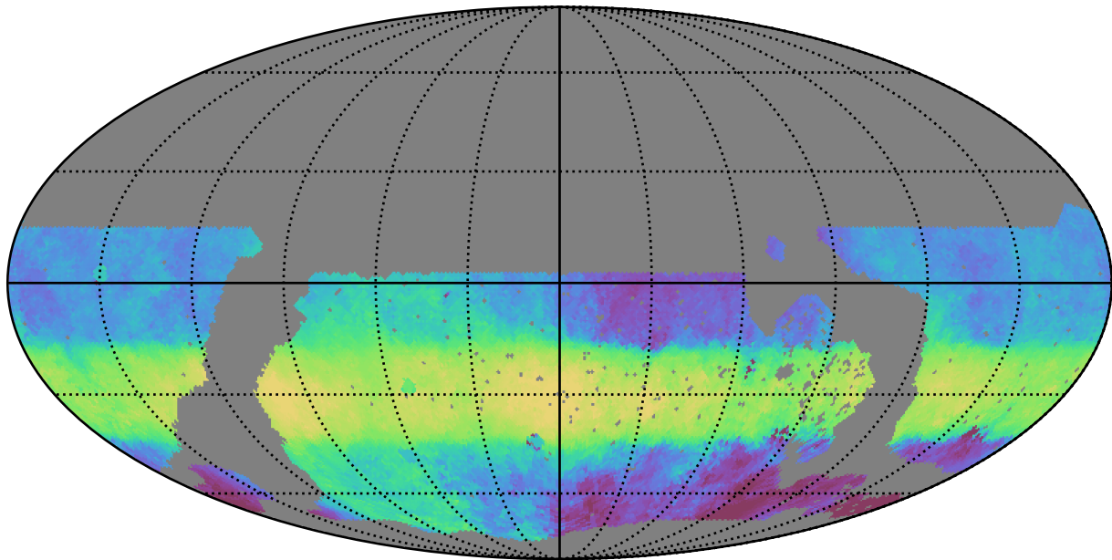
noroll_mjdp60_v3.4_10yrs WFD z band: Median HA
