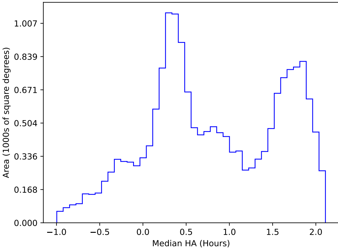
noroll_mjdp60_v3.4_10yrs WFD z band: Median HA
