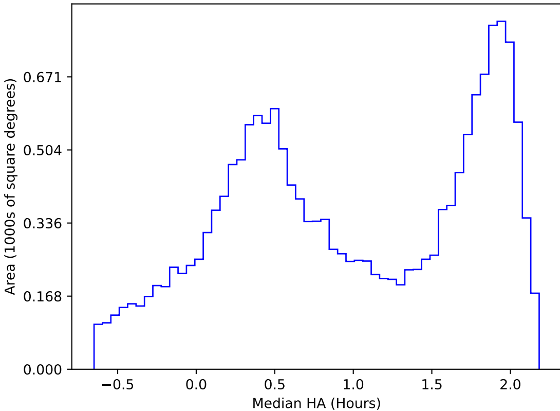
noroll_mjdp60_v3.4_10yrs WFD y band: Median HA
