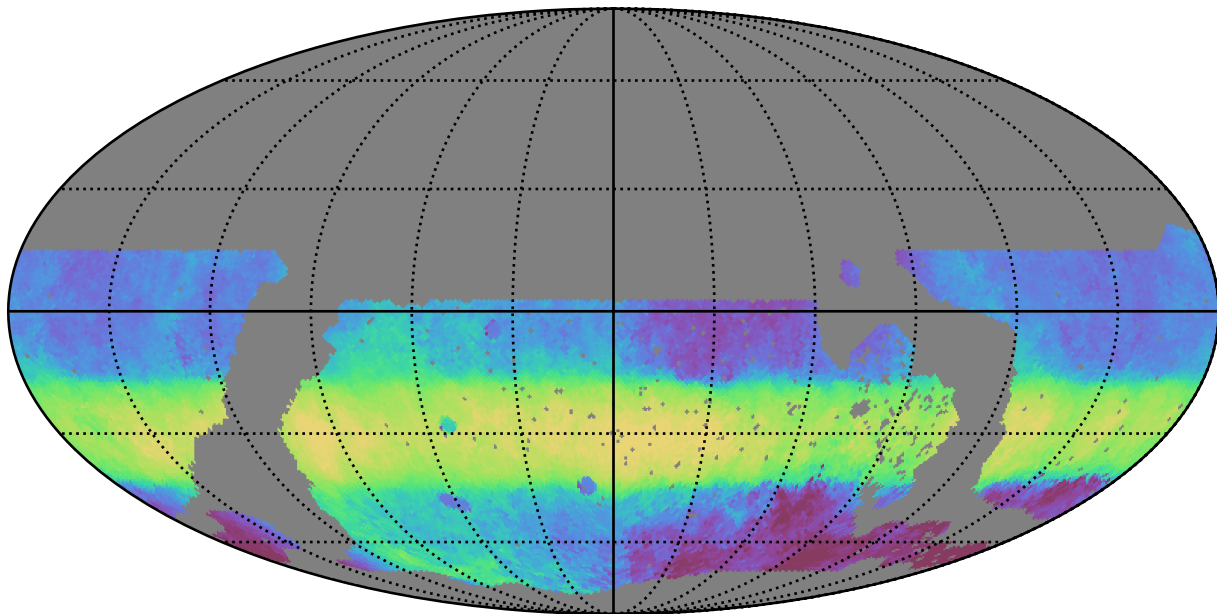
noroll_mjdp60_v3.4_10yrs WFD i band: Median HA
