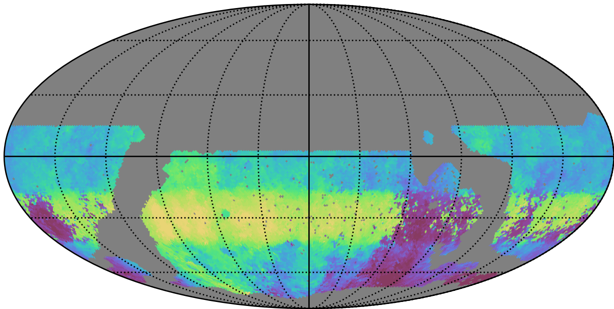
noroll_mjdp60_v3.4_10yrs WFD g band: Median HA
