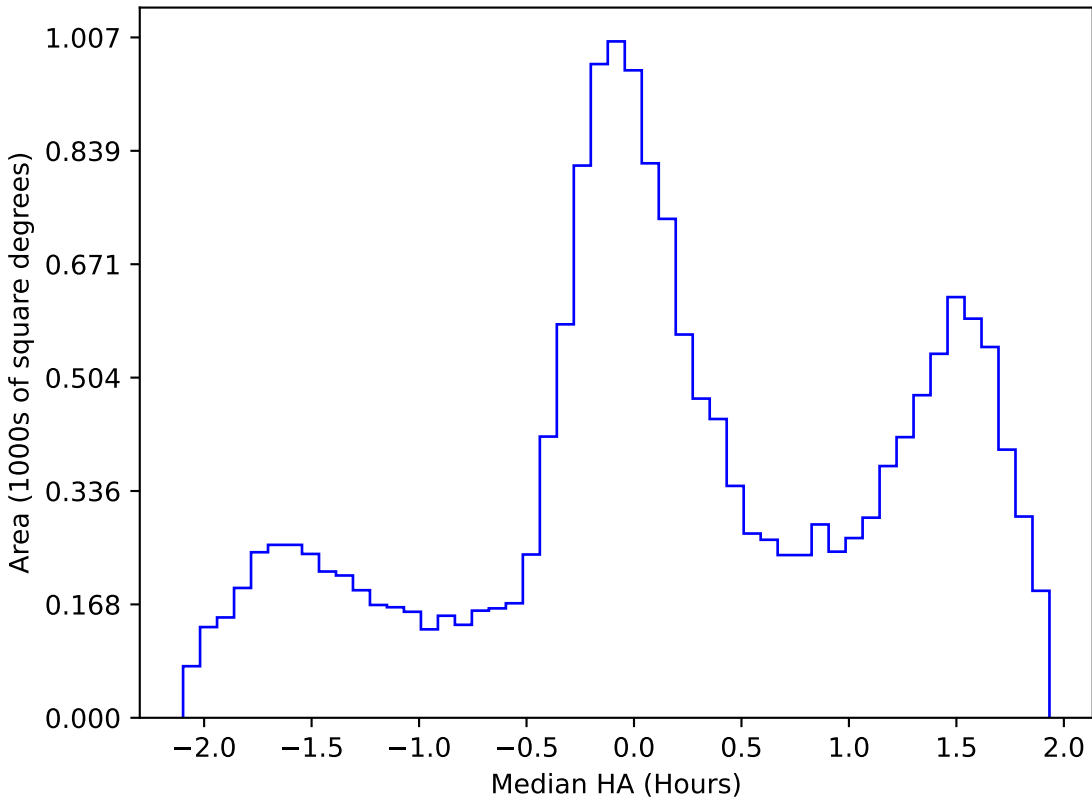
noroll_mjdp60_v3.4_10yrs WFD g band: Median HA
