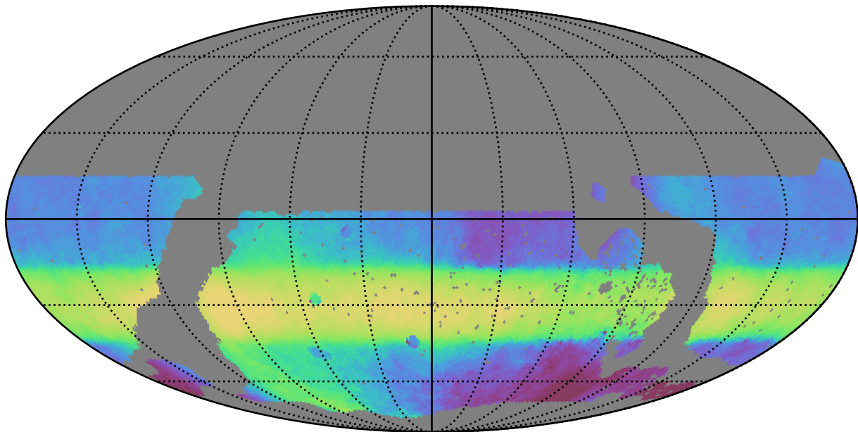
noroll_mjdp60_v3.4_10yrs WFD all bands: Median HA
