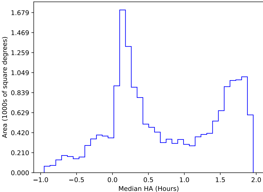
noroll_mjdp60_v3.4_10yrs WFD all bands: Median HA
