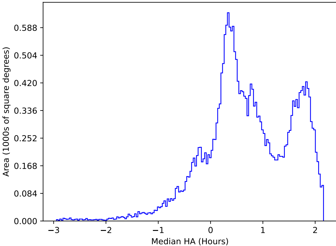
noroll_mjdp60_v3.4_10yrs All sky z band: Median HA
