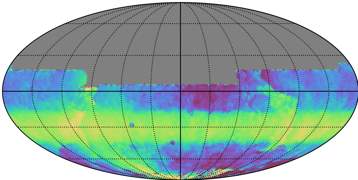
noroll_mjdp60_v3.4_10yrs All sky y band: Median HA
