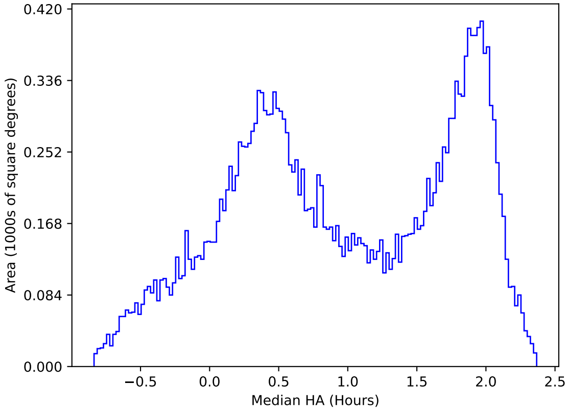
noroll_mjdp60_v3.4_10yrs All sky y band: Median HA
