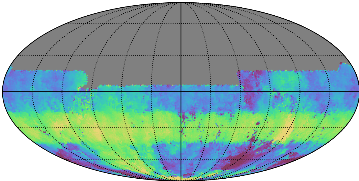
noroll_mjdp60_v3.4_10yrs All sky u band: Median HA
