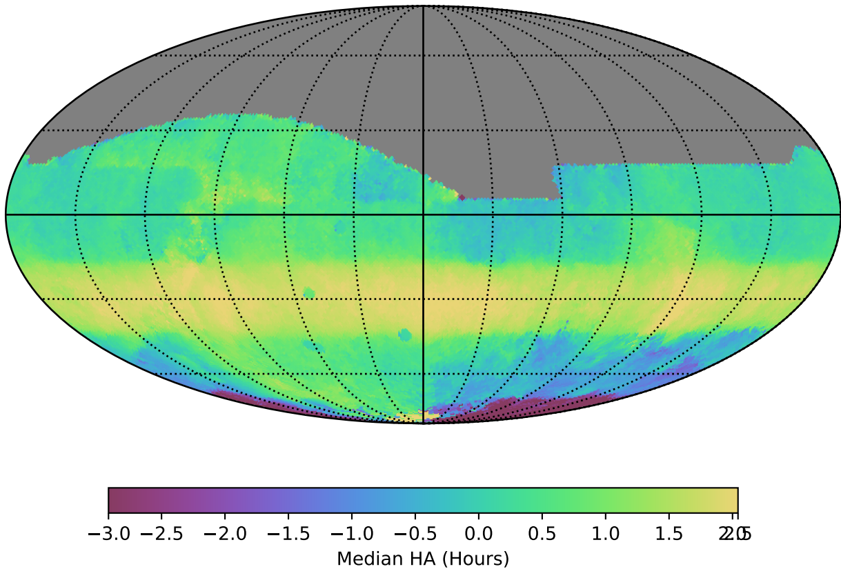
noroll_mjdp60_v3.4_10yrs All sky i band: Median HA
