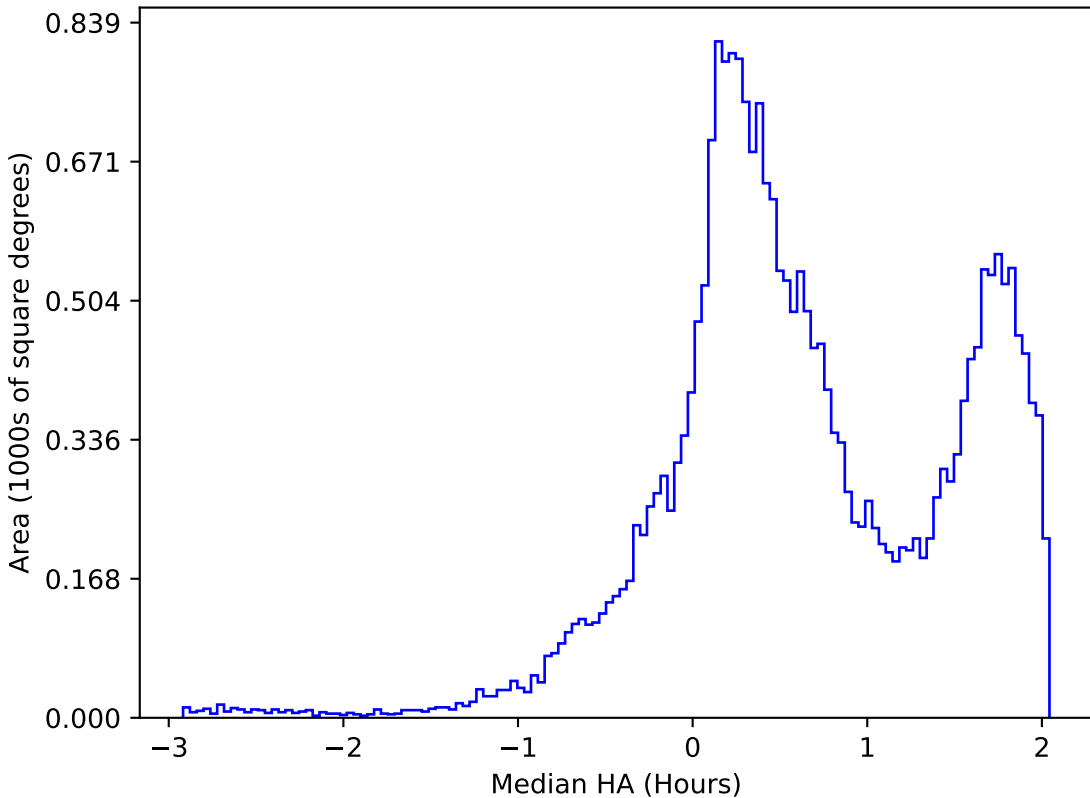
noroll_mjdp60_v3.4_10yrs All sky i band: Median HA
