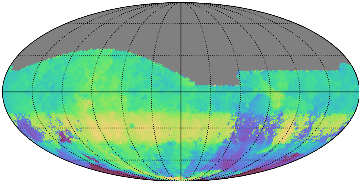
noroll_mjdp60_v3.4_10yrs All sky g band: Median HA
