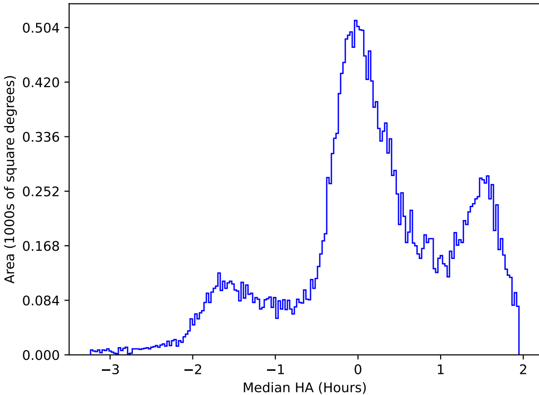
noroll_mjdp60_v3.4_10yrs All sky g band: Median HA
