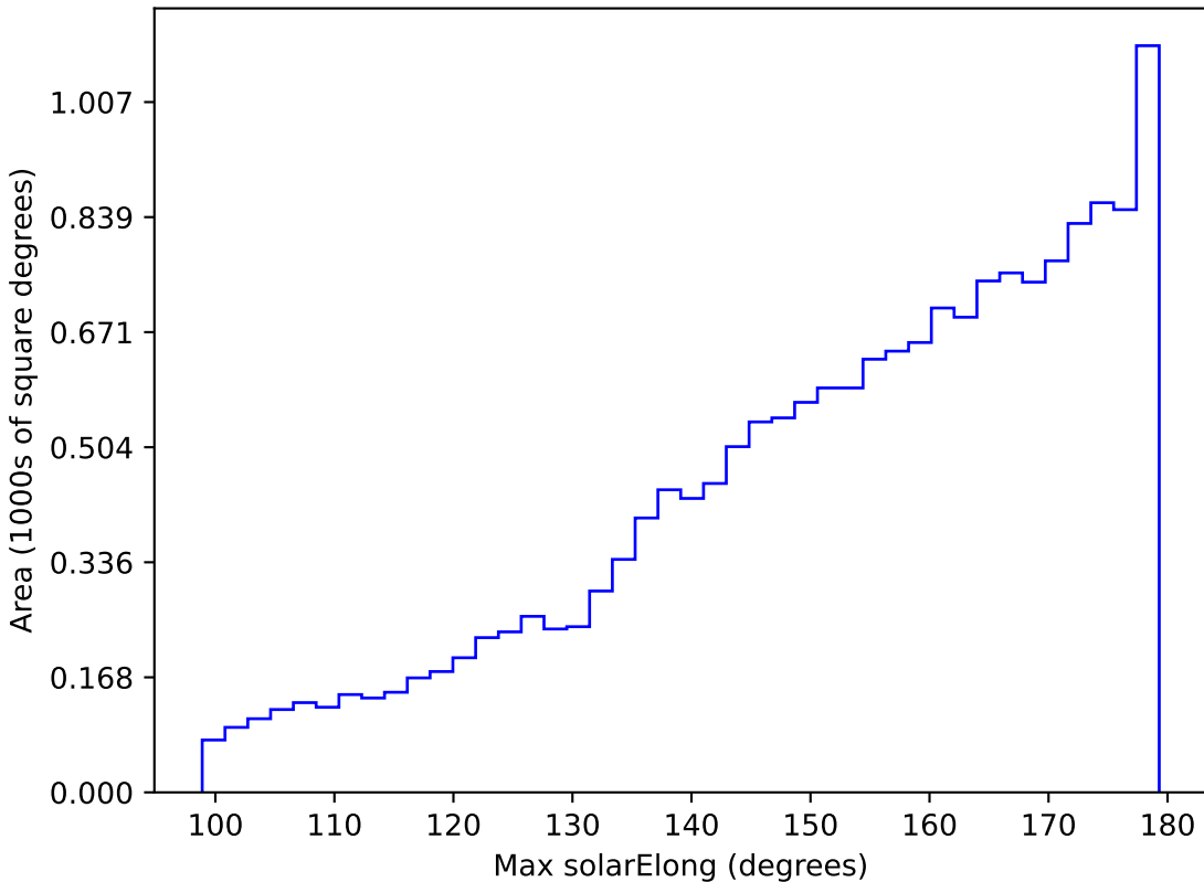
noroll_mjdp60_v3.4_10yrs WFD z band: Max solarElong
