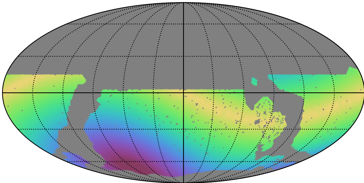
noroll_mjdp60_v3.4_10yrs WFD y band: Max solarElong
