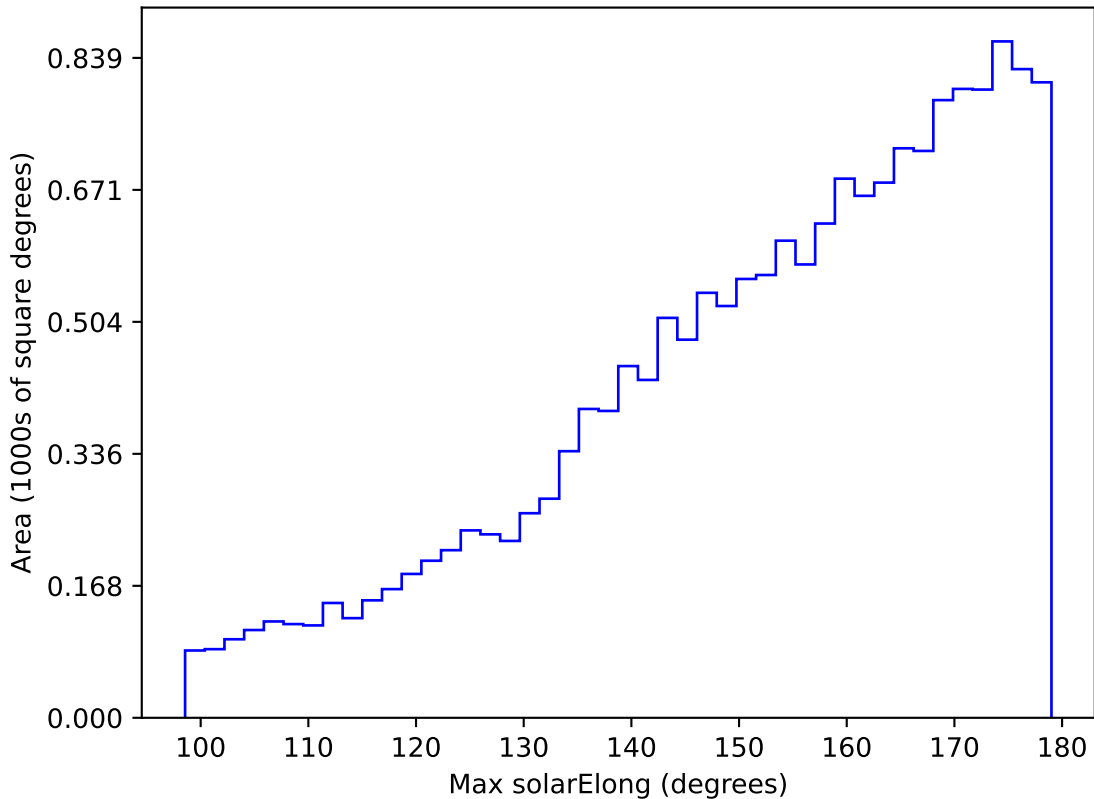
noroll_mjdp60_v3.4_10yrs WFD u band: Max solarElong
