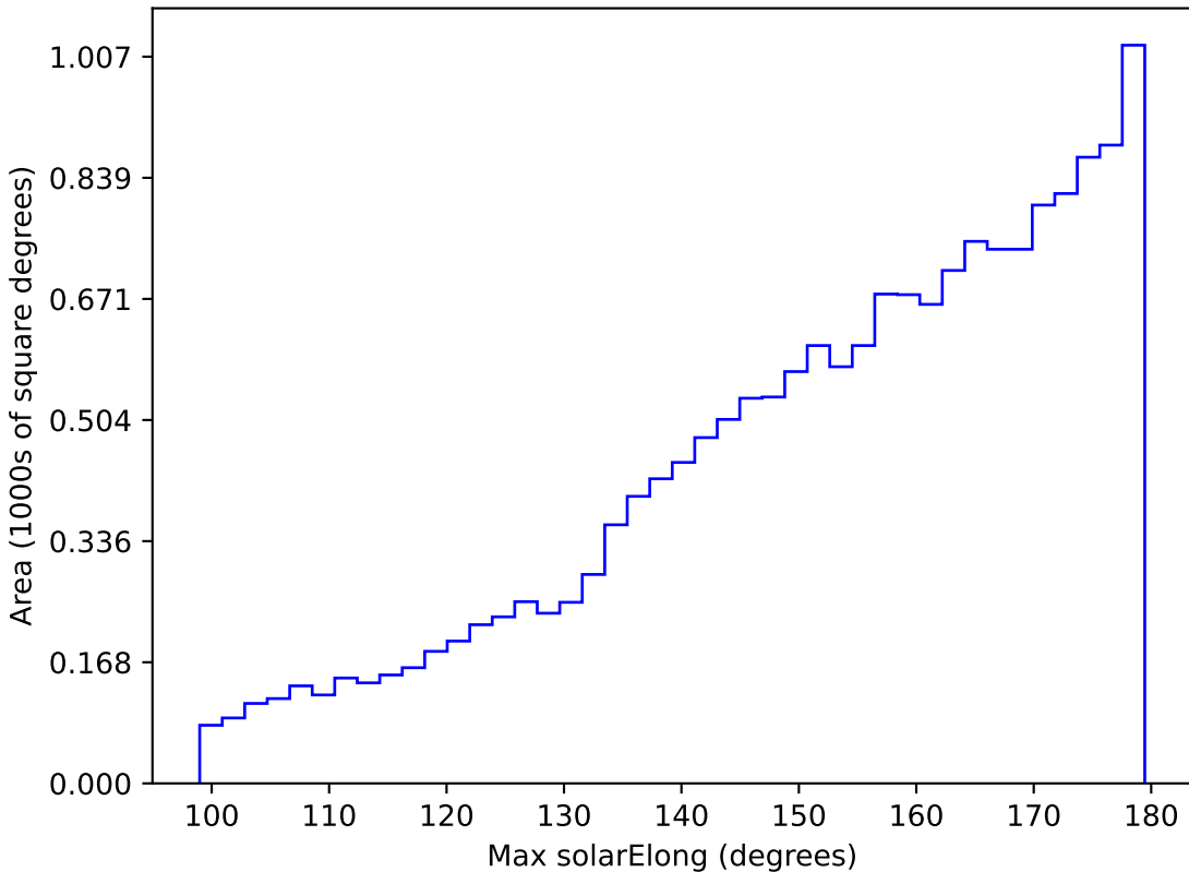
noroll_mjdp60_v3.4_10yrs WFD r band: Max solarElong
