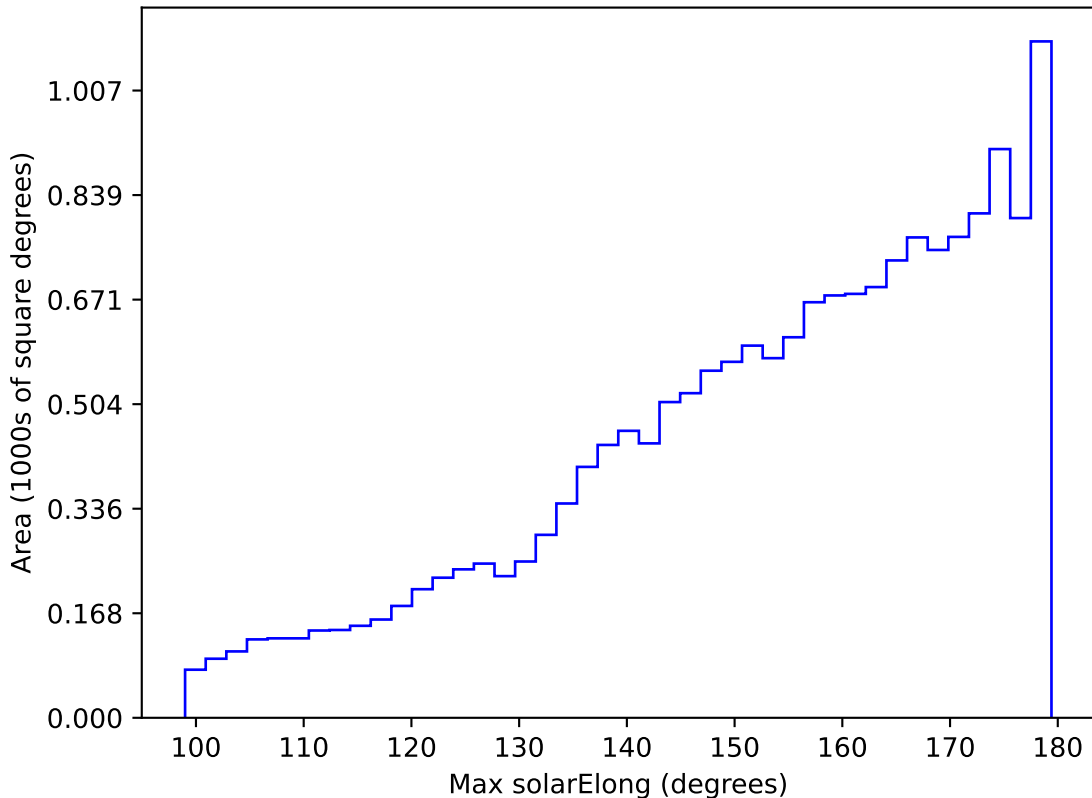
noroll_mjdp60_v3.4_10yrs WFD i band: Max solarElong
