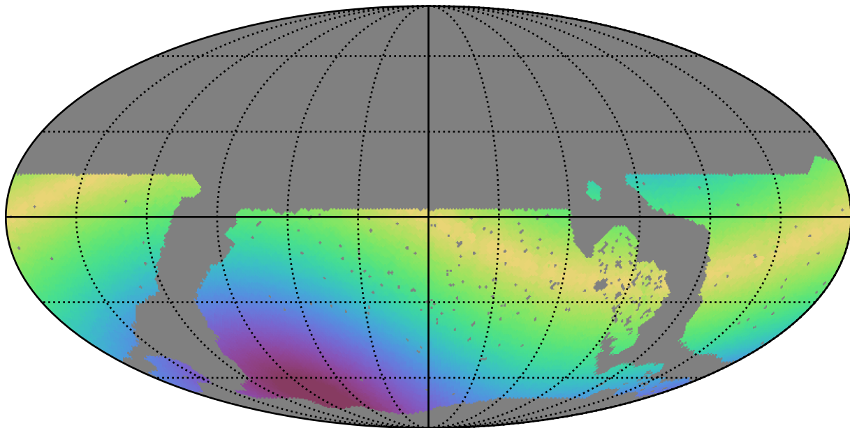
noroll_mjdp60_v3.4_10yrs WFD g band: Max solarElong
