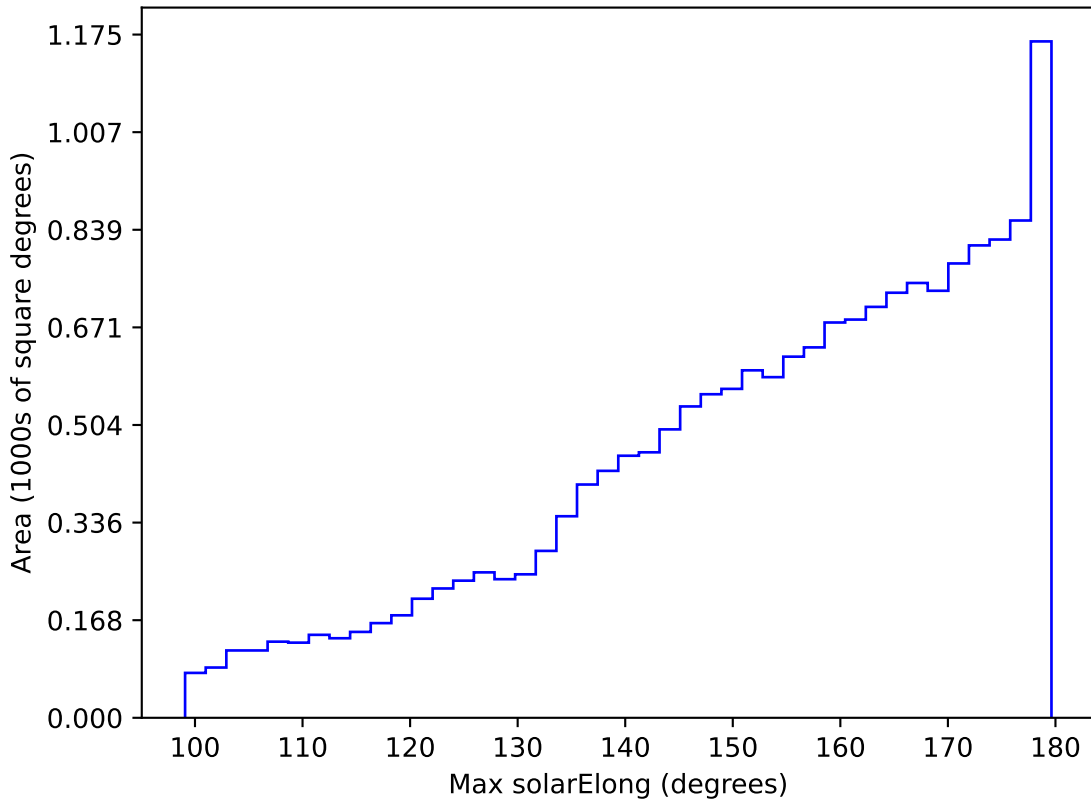
noroll_mjdp60_v3.4_10yrs WFD all bands: Max solarElong
